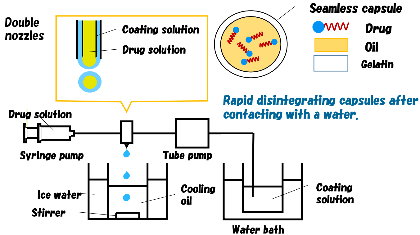
Fig 1. Seamless capsule manufacturing apparatus using double nozzles
